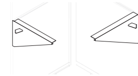
Left Hand Right Hand Wing Wall Bracket (Left hand / Right hand): SYBLWWB
